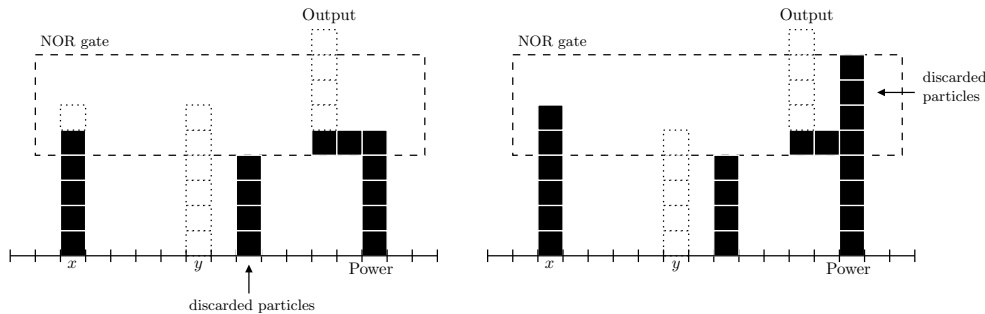
FIG. 12. Left: Evaluation of the wires transmitting values x = \text{TRUE} and y = \text{FALSE} , as well as the power cable. Right: Evaluation of the NOR gate for that case.
