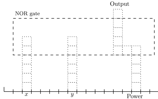
FIG. 10. Skeleton of the construction of a circuit consisting of only one NOR gate.
