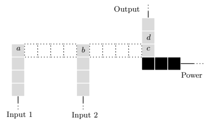
FIG. 5. Gadget for the simulation of a NOR gate. Both inputs are grown until they reach the sites directly below sites a and b , respectively. Two successive particles then follow the path a \rightarrow b \rightarrow c following the dotted line, stopping according to the inputs. The output is then grown from site c .
