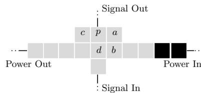
FIG. 8. Gadget for the simulation of an OR gate. The input is grown up to site p . A first particle then follows the trajectory a \rightarrow b , stopping according to the truth value of the gadget's input. Then, a second particle makes the trajectory c \rightarrow d , also stopping according to the truth value of the input. To finalize, the power wire is grown starting from site d , and the output is grown from site p . This OR gate with a single input, in fact, simulates the crossing of the input wire with the power wire.
