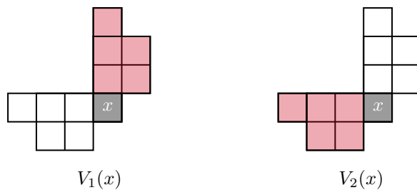
FIG. 26. Visual representation of V(x) . Sets V_1(x) and V_2(x) are highlighted in red. (See online version for color.)
