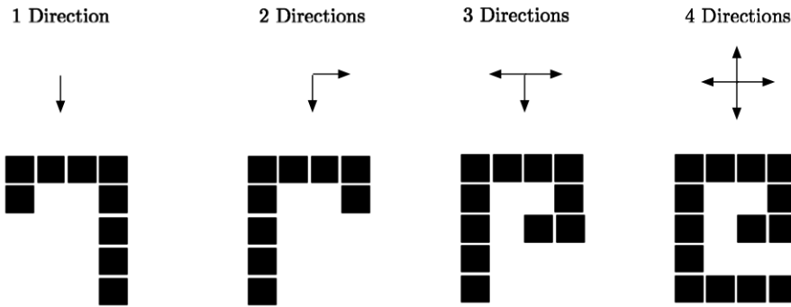
FIG. 18. Four nonconstructible figures with their respective maximum number of directions where they are not constructible. The last figure is not constructible even with four directions.
