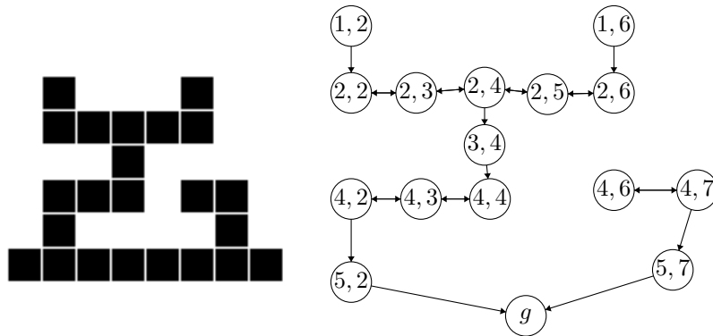
FIG. 19. Shape and graph obtained from sequence S = 2\ 7\ 7\ 2\ 6\ 3\ 4\ 4\ 4\ 5\ 6\ 3\ 2\ 6\ 2 .
