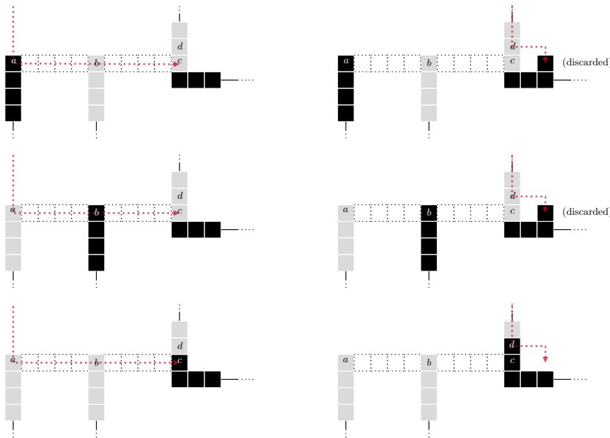
FIG. 6. Examples of the dynamics of a NOR gate when one of the two inputs is TRUE (top and middle rows) and when both inputs are FALSE (bottom row). The three lines in the left column depict as a red pointed line the trajectory of the particle that follows a \rightarrow b \rightarrow c . Notice that in the first and second lines the particle is fixed before reaching position c , while in the third line the particle reaches position c . The right column also depicts the trajectory of the wire that grows from d , which is only fixed in that position in the third line. (See online version for color.)
